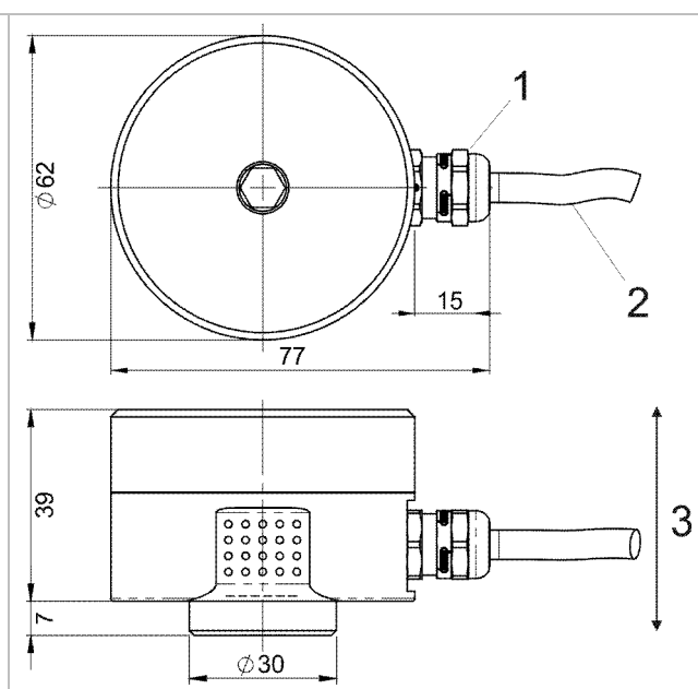
Fig. 5: Housing with integrated cable
