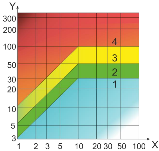
Fig. 8: Vibration intensity diagram [DIN ISO 13373-3]
